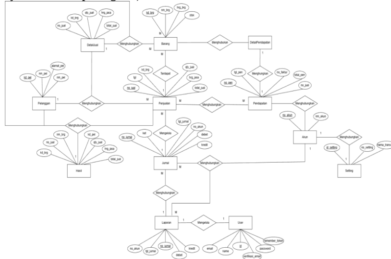
Gambar 2 ERD Penelitian
