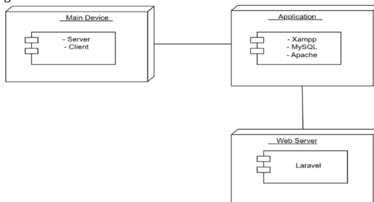
Gambar 3 Deployment Diagram
