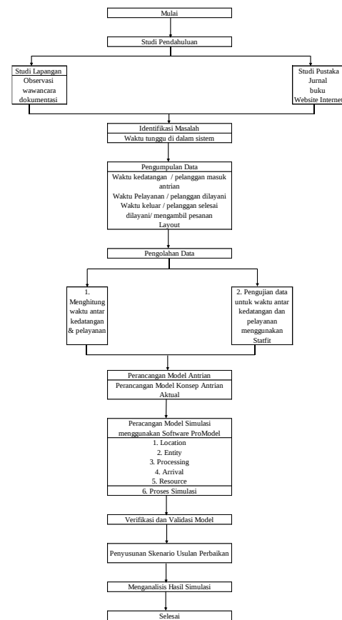
Gambar 1. Model Konseptual
