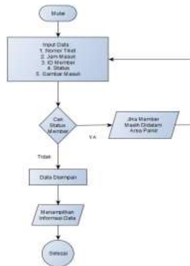
Gambar 2. Flowchart Diagram Parkir Masuk
