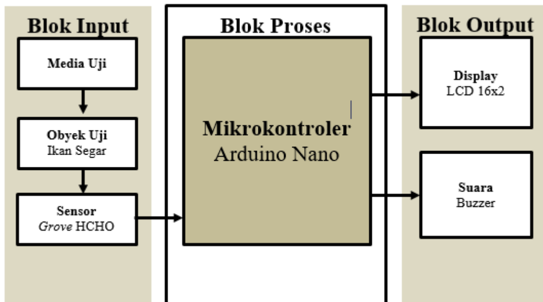
Gambar. Blok diagram alat
